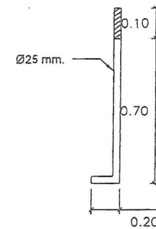
DETAIL ANCHOR BOLT
